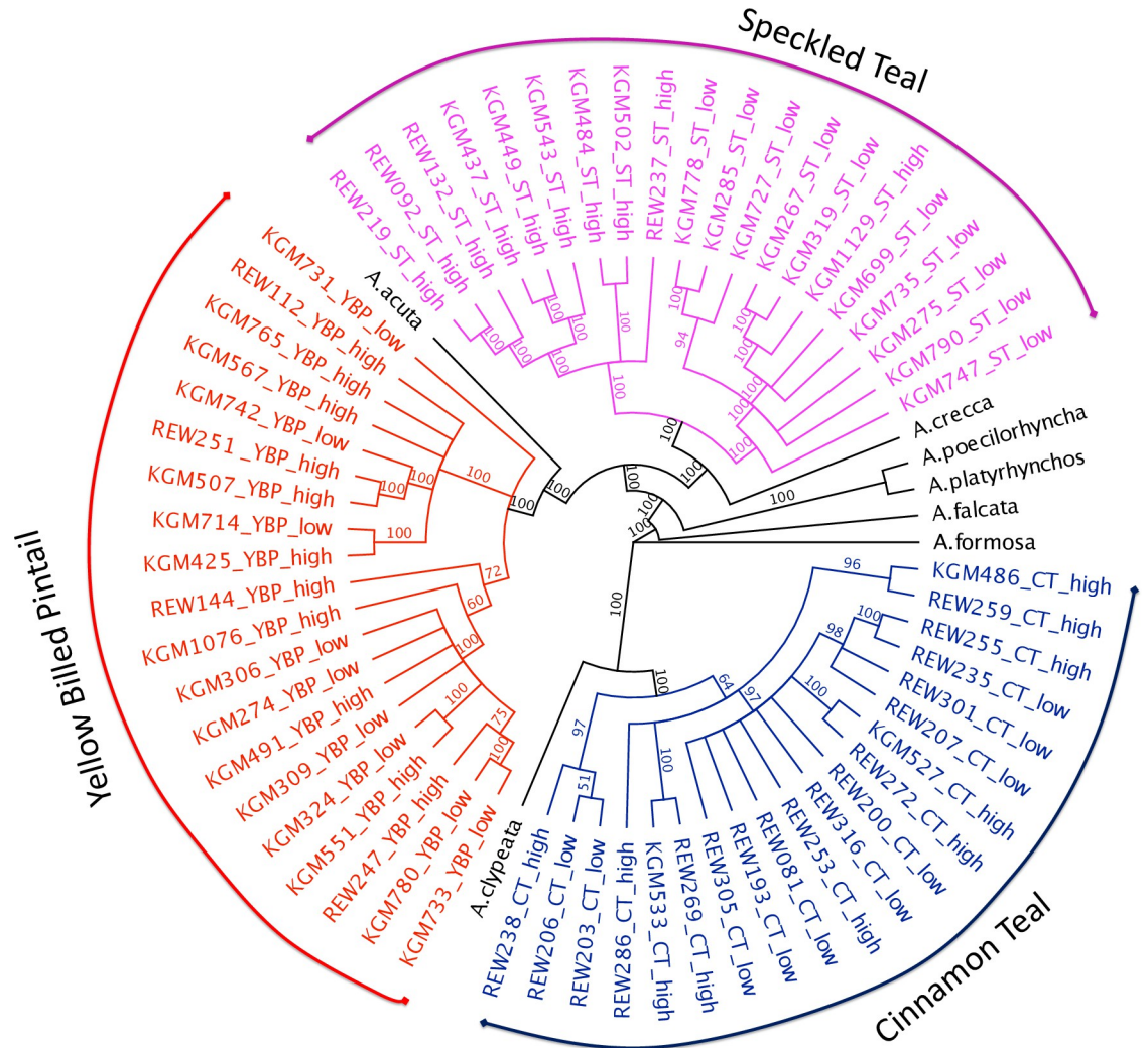
Fig 2. Maximum-likelihood tree (GARLI) using the full mitochondrial genomes of the speckled teal (pink), yellow-billed pintail (red) and cinnamon teal (blue), along with other Anas outgroups. Numbers at nodes represent percent consensus support; “high” = individuals from high-altitude populations, “low” = individuals from low-altitude populations.
