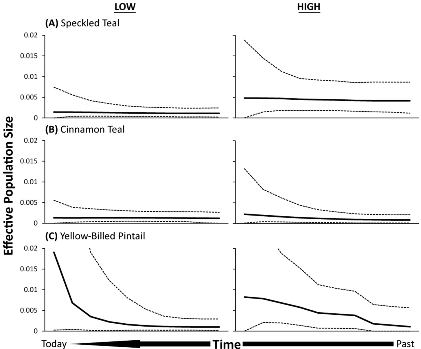
Fig 3. Bayesian skyline plots for low- and high-altitude populations of (A) speckled teal, (B) cinnamon teal, and (C) yellow-billed pintail.
