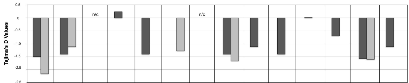
Fig 5. Tajima's D for the individual protein-coding genes across each high- (dark grey) and low-altitude population (light grey) of the three species; nc = not calculated, due to a lack of nucleotide variation.
