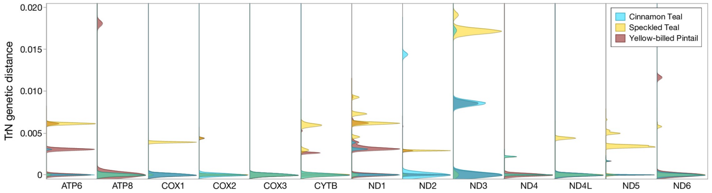
Fig 4. Kernal density plots showing pairwise distances between low- and high-altitude populations of each species calculated for each mitochondrial protein-coding gene using the Tamura-Nei (TrN) model of nucleotide substitution.
